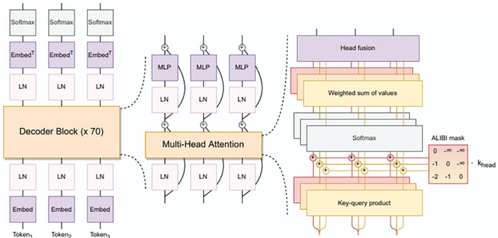
Fig. 9. The BLOOM architecture example sourced from [13].
