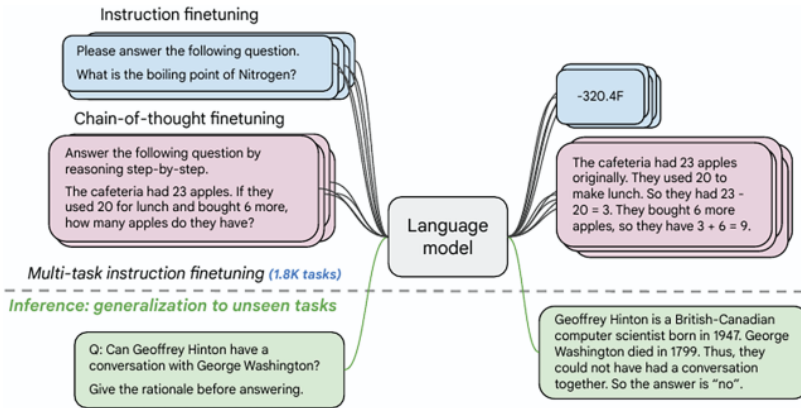
Fig. 11. An example image shows an instance of the Flan training paradigm, taken from [16].
