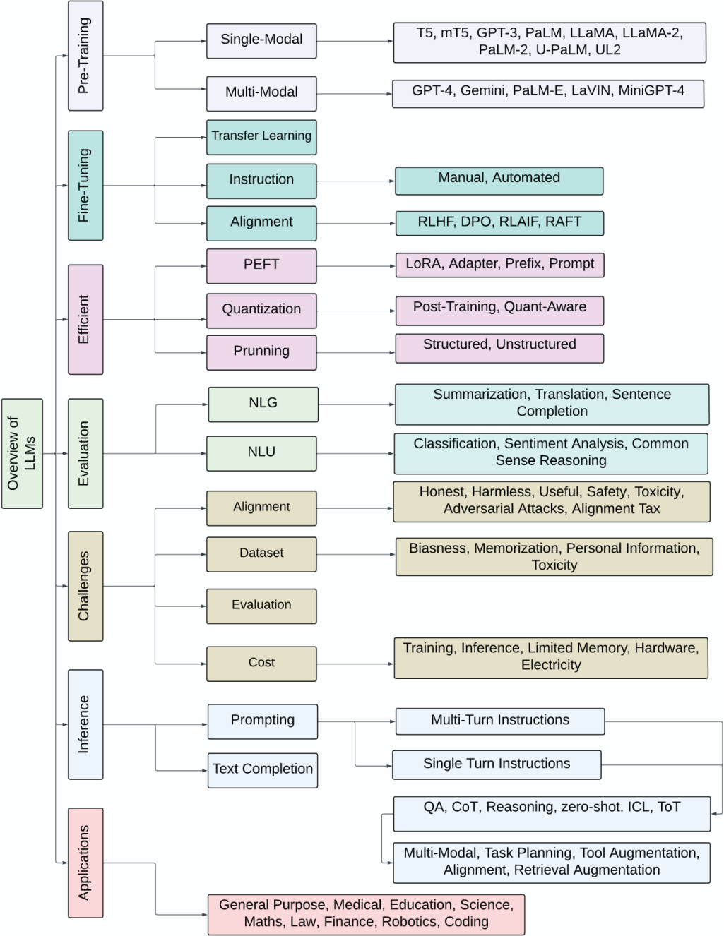
Fig. 3. A broader overview of LLMs, dividing LLMs into seven branches: (1) pre-training, (2) fine-tuning, (3) efficient, (4) inference, (5) evaluation, (6) applications, and (7) challenges.
