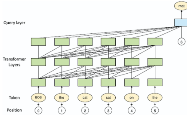
Fig. 8. The image is the article of [111], showing an example of PanGu- \alpha architecture.
