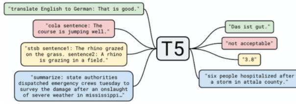
Fig. 7. Unified text-to-text training example, source image from [10].
