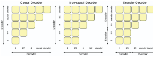
Fig. 4. An example of attention patterns in language models, image is taken from [93].
