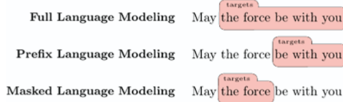
Fig. 5. An example of language model training objectives, image from [93].
