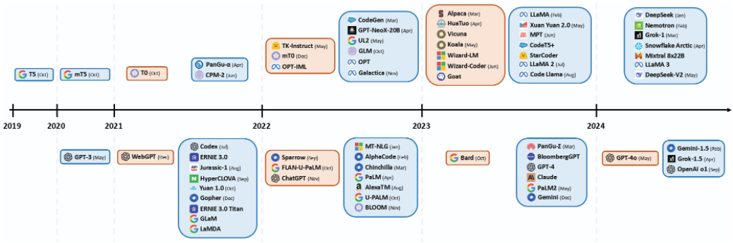
Fig. 2. Chronological display of LLM releases: blue cards represent “pre-trained” models, while orange cards correspond to “instruction-tuned” models. Models on the upper half signify open-source availability, whereas those on the bottom are closed-source. The chart illustrates the increasing trend toward instruction-tuned and open-source models, highlighting the evolving landscape and trends in NLP research.
