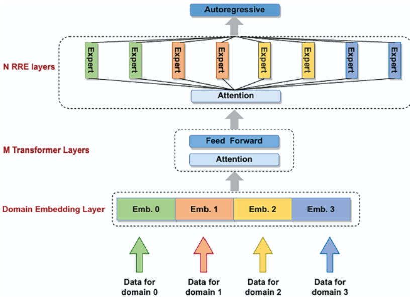
Fig. 10. This example illustrates the PanGu-Σ architecture, as depicted in the image sourced from [92].
