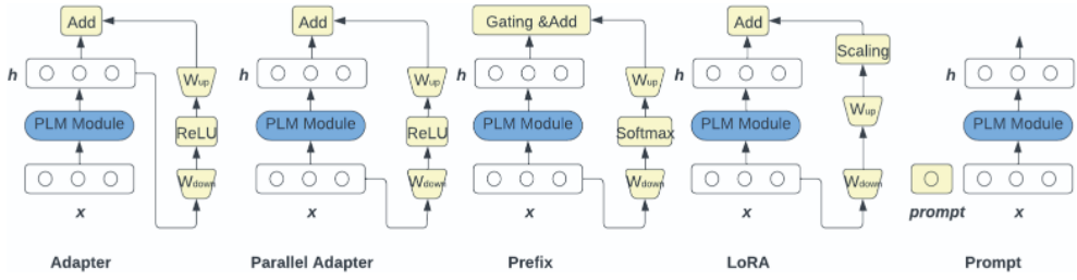
Fig. 14. Illustration of parameter-efficient fine-tuning paradigms, where x is input and h is hidden state, figure courtesy [38]. Parallel adapter and low-rank adaptation (LoRA) fall in the adapter tuning category.
